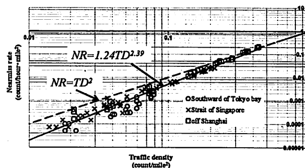
Figure 9. The traffic volume allowance degree
