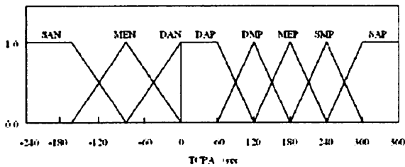
Figure 1. Membership function for TCPAc or TCPAv
