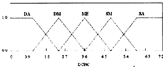
Figure 2. Membership function for DCPA'
