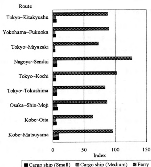
Fig. 2 Comparison of cost (Truck=100)
