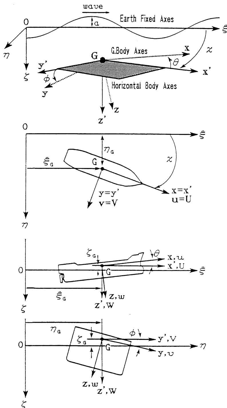
Fig. 23 Co-ordinate systems
